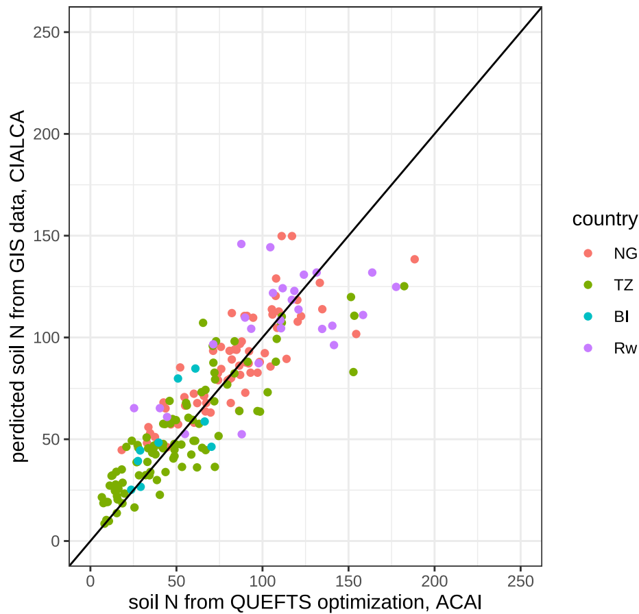
Soil Grids + control class, AC and CI data together
